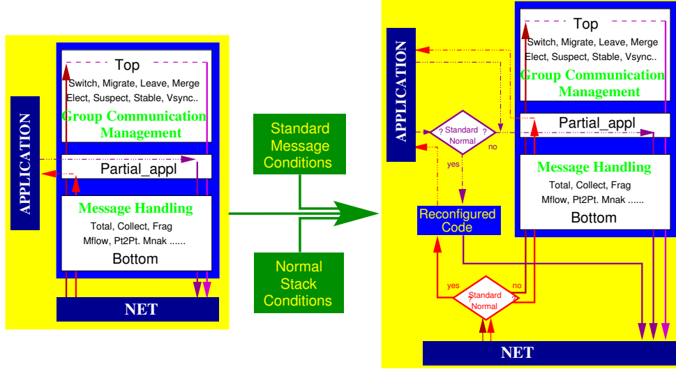
Fig. 19. Stack reconfiguration including the partial_appl layer
