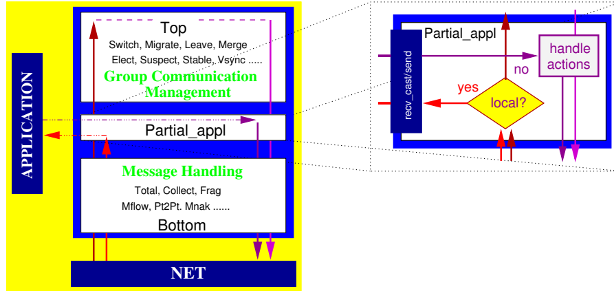
Fig. 15. Application messages leave the stack in the partial_appl layer
